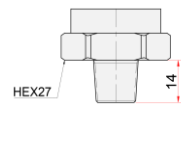
R1/4" ISO 7
