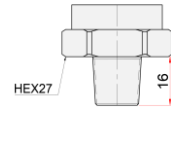
R3/8" ISO 7
