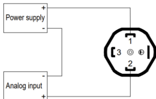
2-wire / current
