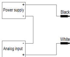
2-wire / current
