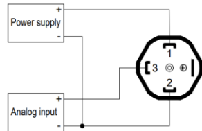
3-wire / voltage
