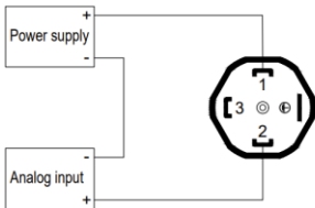
2-wire / current
