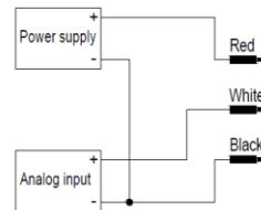
3-wire / voltage
